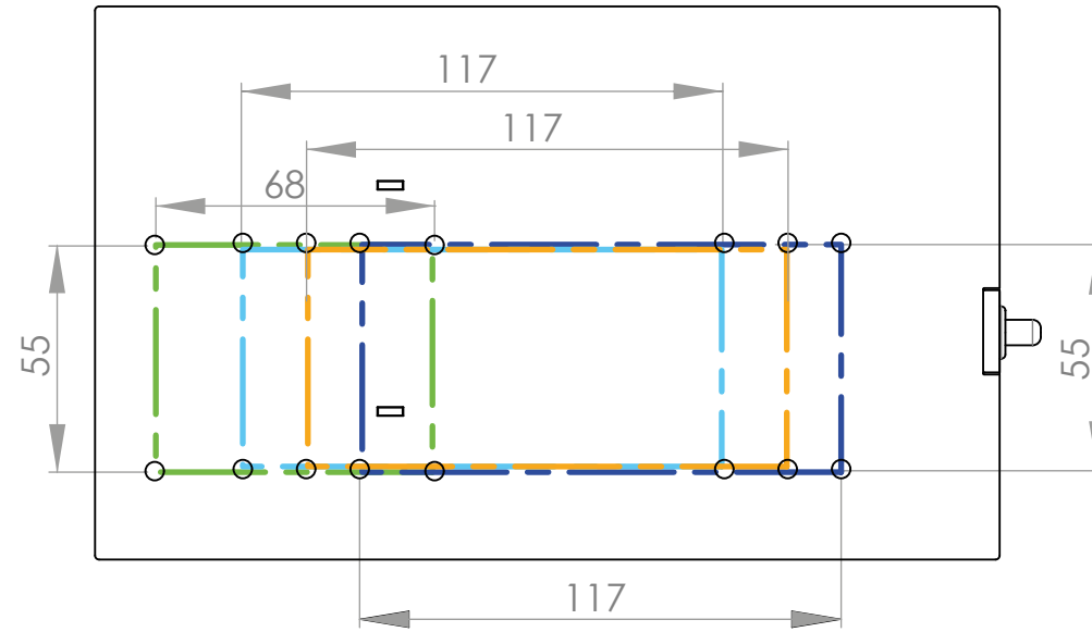
Removable plate for throttle controls
